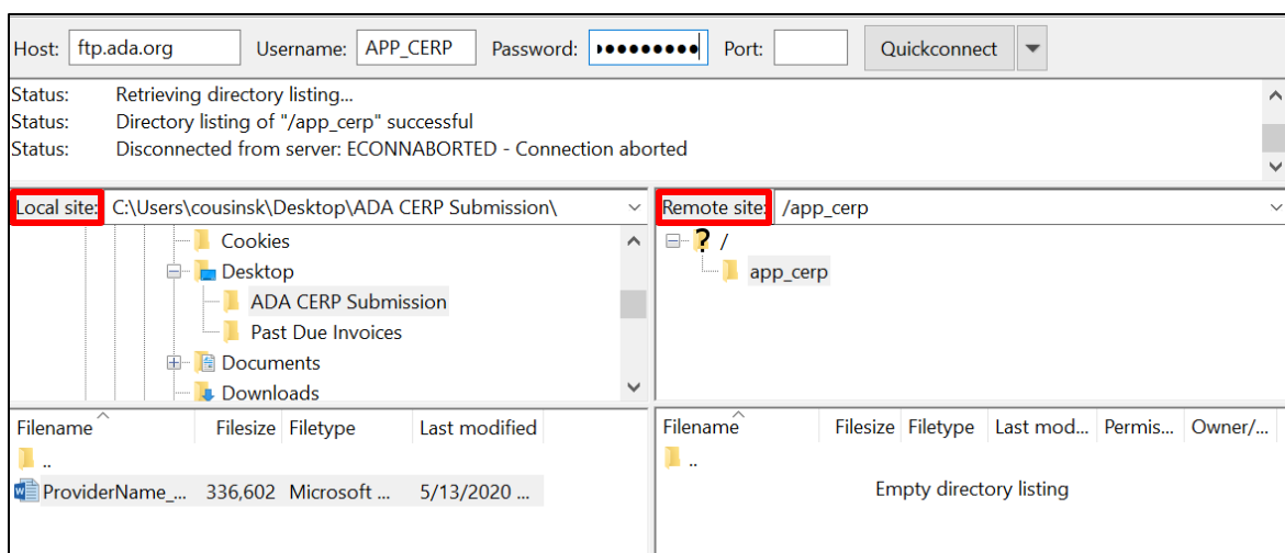
Figure 2. FileZilla view
